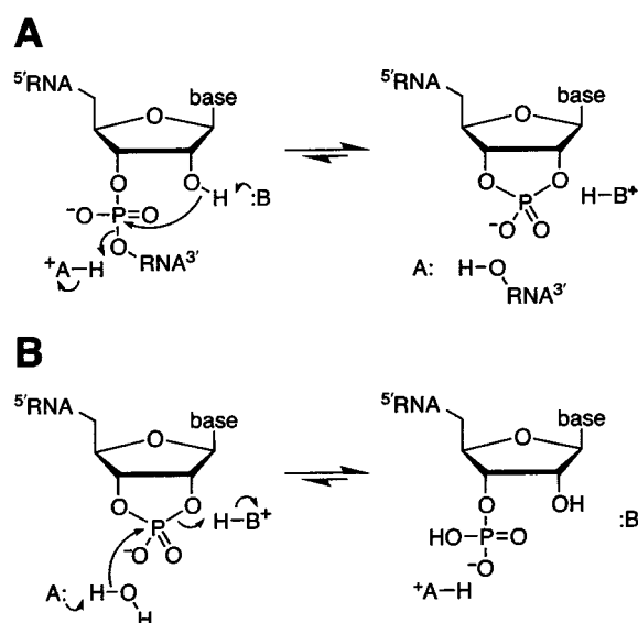
FIGURE 1: Putative mechanism of catalysis by ribonuclease A (3, 4). (A) Transphosphorylation reaction. (B) Hydrolysis reaction. In both panels, B and A refer to His12 and His119, respectively.
