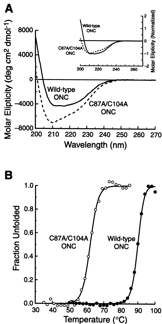
Fig. 2. Conformation and conformational stability of wild-type Onconase ® and the C87A/C104A variant in PBS. A: CD spectrum of wild-type Onconase ® (solid line) and C87A/C104A Onconase ® (broken line) at 25°C. Inset: spectra normalized using the molar ellipticity at 210 nm as a reference. B: Thermal unfolding of wild-type Onconase ® (●) and the C87A/C104A variant (○) monitored by CD spectroscopy at 204 nm. Data for wild-type Onconase ® are from [9].
