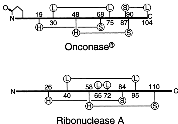
Fig. 1. Connectivity of the disulfide bonds in Onconase ® (104 residues) and ribonuclease A (124 residues). The secondary structural context of each half-cystine residue is indicated by H ( \alpha -helix), S ( \beta -sheet) or L (loop). The N-terminal residue of Onconase ® is a pyrrolutamate.
