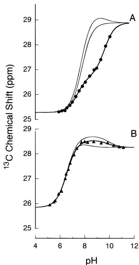
FIGURE 5: Fit of experimental data to titration curves with dependent pK_a 's (eq 3). (A) Wild-type thioredoxin (Trx). (B) CVWC Trx. The pK_a and ^{13}\text{C} chemical shift values are listed in Table 3. The other curves are fits of the experimental data to eq 3, assuming that c = 1 and that the pK_a of Asp26 is always 7.5 (lower curve) or 9.2 (upper curve).
