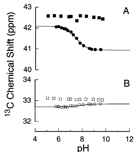
FIGURE 2: The pH dependence of the 13 C β signals from oxidized [ 13 C β -Cys]thioredoxins in D 2 O. (A) Cys32 in wild-type thioredoxin (Trx; ●) and D26L Trx (■). (B) Cys35 in wild-type Trx (○) and D26L Trx (□). Titrations were carried out at 308 K in 0.1 M potassium phosphate buffer.
