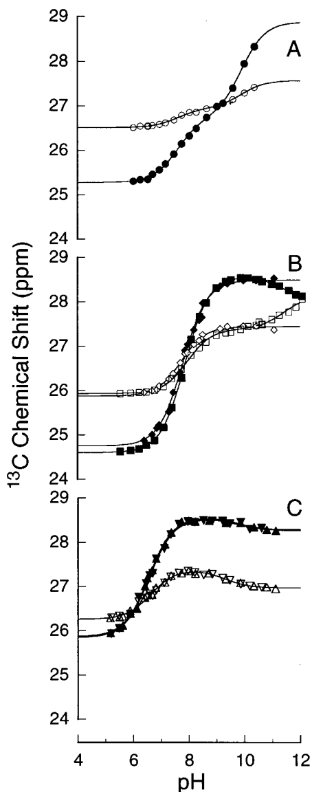
FIGURE 3: The pH dependence of the ^{13}\text{C}^{\beta} signals from reduced [ ^{13}\text{C}^{\beta} -Cys]thiothioredoxins in \text{D}_2\text{O} . Closed symbols, Cys32; open symbols, Cys35. (A) Wild-type thiothioredoxin (Trx; ●, ○). (B) D26L Trx (■, □) and D26N Trx (◆, ◇). (C) CWGC Trx (▲, △) and CVWC Trx (▼, ▽). The \text{pK}_a values determined from fitting the experimental data to eq 2 are listed in Table 2. Titrations were carried out at 308 K in 0.1 M potassium phosphate buffer containing DTT (5.0 mM).
