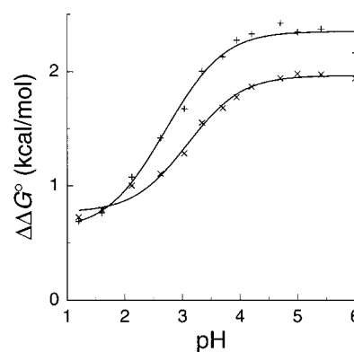
FIGURE 6: Plot of \Delta\Delta G^\circ (= \Delta G^\circ_{\text{wild-type}} - \Delta G^\circ_{\text{D121N/A}}) versus pH for D121N ribonuclease A (x) and D121A ribonuclease A (+). Values of \Delta G^\circ were calculated from values of \Delta H_m using regression analysis of \Delta H_m versus T_m . The lines are nonlinear least-squares fits of the data to eq 8, using the parameters pK_U = 3.5 , pK_N = 2.6 , and \Delta\Delta G^\circ([H^+] = \infty) = 0.78 kcal/mol for D121N RNase A; and pK_U = 3.3 , pK_N = 2.1 , and \Delta\Delta G^\circ([H^+] = \infty) = 0.62 kcal/mol for D121A RNase A.
