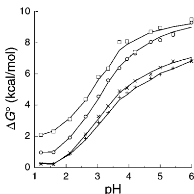
FIGURE 5: Plot of \Delta G^\circ versus pH for wild-type ribonuclease A (O) and the D121N (x), D121A (+), and H119A (□) variants. The points were calculated from the observed \Delta H_m values using eq 3. The lines were calculated by using \Delta H_m values from regression analysis of \Delta H_m versus T_m .
