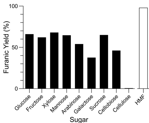
Fig. 4 Bar graph showing the effect of sugar type on furanic yield as catalyzed by 2-CPBA. HMF was recovered quantitatively, indicating its stability under the reaction conditions. Reaction conditions are as follows: 1.0 mL of DMSO containing a sugar (10% w/v), [BMIM]Cl (0.19 M), and 2-CPBA (1 equiv.); shaken (650 rpm) at 95 °C for 1 h
