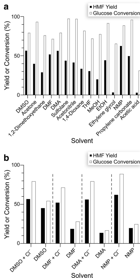
Fig. 3 Bar graphs showing the effect of solvent and chloride ion on the yield of HMF and conversion of glucose as catalyzed by 2-CPBA. a Higher selectivity is obtained in polar aprotic solvents that are strong electron donors, such as a DMSO, DMF, DMA, and NMP. Reaction conditions are as follows: 1.0 mL of a solvent containing glucose (10% w/v), [BMIM]Cl (0.19 M), and 2-CPBA (1 equiv.); shaken (650 rpm) at 95 °C for 1 h. b In DMSO, DMF, DMA, and NMP, a higher HMF yield and glucose conversion is obtained in the presence of chloride ion. Reaction conditions are as follows: 1.0 mL of a solvent containing glucose (10% w/v) and 2-CPBA (1 equiv.), with or without [BMIM]Cl (0.19 M); shaken (650 rpm) at 95 °C for 1 h. Data with [BMIM]Cl are reproduced from panel A to facilitate comparisons
