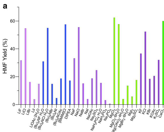
Fig. 2 Bar graphs showing the yield of HMF from glucose in DMSO containing different salts as catalyzed by 2-CPBA. a Salts grouped by cation. b Salts grouped by anion. Bars are rendered in CPKnew colors for
