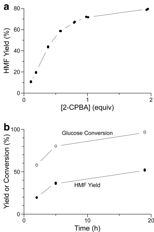
Fig. 5 Catalysis of the conversion of glucose to HMF by 2-CPBA. a Graph of HMF yield as a function of 2-CPBA concentration. Reaction conditions are as follows: 1.0 mL of DMSO containing glucose (10% w/v), [BMIM]Cl (0.19 M), and 2-CPBA (0.11–1.95 equiv.); shaken (650 rpm) at 95 °C for 2 h. b Graph of HMF yield and glucose conversion afforded by 2-CPBA (0.2 equiv.) as a function of time ( n = 2 ). Reaction conditions are as follows: 1.0 mL of DMSO containing glucose (10% w/v), [BMIM]Cl (0.19 M), and 2-CPBA; shaken (650 rpm) at 95 °C for 2, 5, or 19 h
