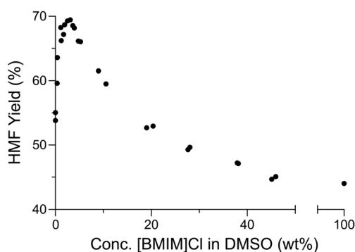
Fig. 1 Graph showing the effect of [BMIM]Cl concentration on the yield of HMF in DMSO. Reaction conditions are as follows: 1.0 mL of DMSO containing glucose (10% w/v), [BMIM]Cl, and 2-CPBA (1 equiv.); shaken (650 rpm) at 95 °C for 1 h
