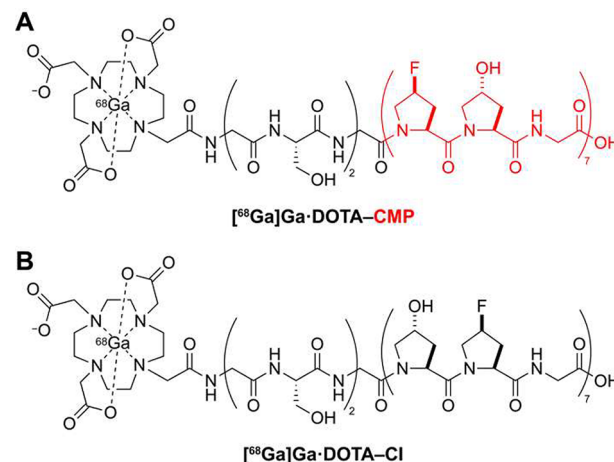
Figure 2. (a) Structure of [ 68 Ga]Ga·DOTA–CMP. The CMP segment is depicted as a red ribbon. (b) Structure of [ 68 Ga]Ga·DOTA–CI.
