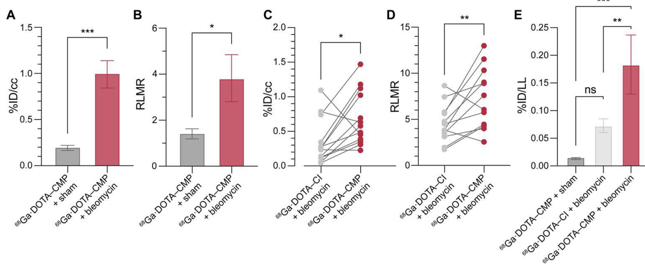
Figure 4. Radiation signal in organs from sham and bleomycin-injured mice injected with [ ^{68}\text{Ga} ]Ga-DOTA–CMP or [ ^{68}\text{Ga} ]Ga-DOTA–CI. (A) In vivo %ID/cc values in right lungs, 50–60 min postinjection as measured by PET. (B) In vivo right lung:muscle ratios (RLMRs), 50–60 min postinjection as measured by PET. In panels A and B, n = 6 for [ ^{68}\text{Ga} ]Ga-DOTA–CMP + sham and n = 5 for [ ^{68}\text{Ga} ]Ga-DOTA–CMP + bleomycin. (C and D) Data from a paired study, in which mice were injected with [ ^{68}\text{Ga} ]Ga-DOTA–CMP and imaged and then 24 h later, injected with [ ^{68}\text{Ga} ]Ga-DOTA–CI and imaged. (C) In vivo %ID/cc values in right lungs 50–60 min postinjection as measured by PET. Connecting lines indicate associated data points from individual animals. (D) In vivo RLMRs 50–60 min postinjection as measured by PET. Connecting lines indicate associated data points from individual animals. (E) Ex vivo %ID/LL in left lung uptake, 90 min postinjection. In panel E, n = 6 for [ ^{68}\text{Ga} ]Ga-DOTA–CMP + sham, 13 for [ ^{68}\text{Ga} ]Ga-DOTA–CI + bleomycin, and 5 for [ ^{68}\text{Ga} ]Ga-DOTA–CMP + bleomycin. An unpaired t test was performed on the data in panels A and B. A paired t test was performed on the data in panels C and D. A one-way ANOVA with a posthoc Tukey test was performed on the data in panel E. Values are the mean \pm SE; *, P < 0.05 ; **, P < 0.01 ; ***, P < 0.001 .
