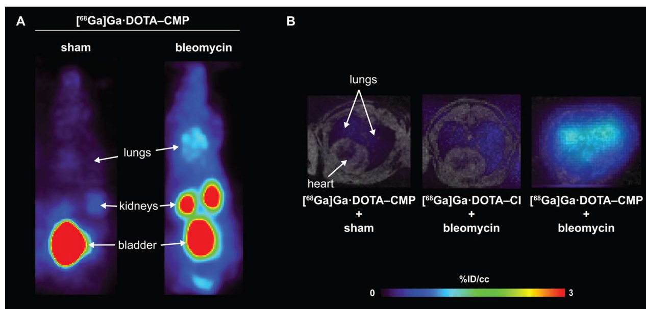
Figure 3. PET and fused PET–MR images of sham and bleomycin-injured mice 50–60 min after tail-vein injection with [ ^{68}\text{Ga} ]Ga-DOTA–CMP or [ ^{68}\text{Ga} ]Ga-DOTA–CI. (A) Representative coronal maximum-in-projection (MIP). (B) Representative axial fused PET (color scale)–MR (gray scale) images of the lungs and heart.
