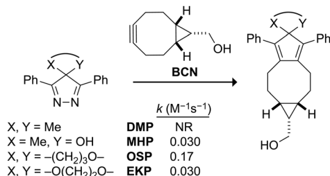
Fig. 1 Reactivity of 4H-pyrazoles in a Diels–Alder reaction. Second-order rate constants were measured in 9:1 methanol/water at 26 °C by HPLC. Values are the mean from triplicate experiments. The value for DMP is from ref. 18; NR, no reaction.
